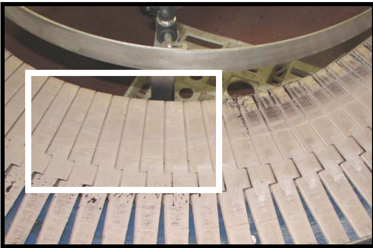
UltraVapor easily cleans ink from the framework and conveyor belt. Floor suction tool used to remove ink on floor that came off framework and conveyor.
